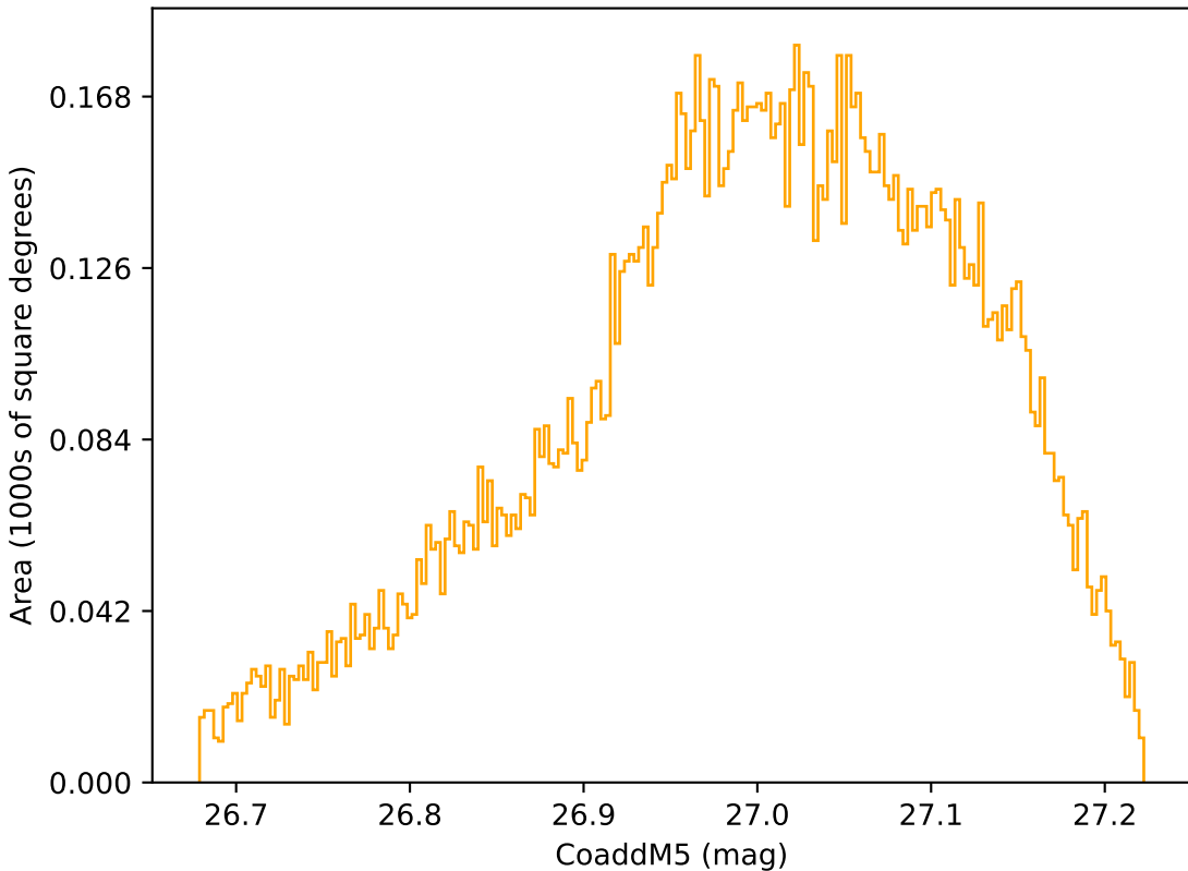
too_ignore_5_4v3.4_10yrs WFD r band: CoaddM5
