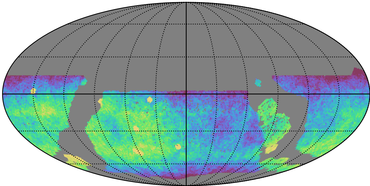
too_ignore_5_4v3.4_10yrs WFD g band: CoaddM5
