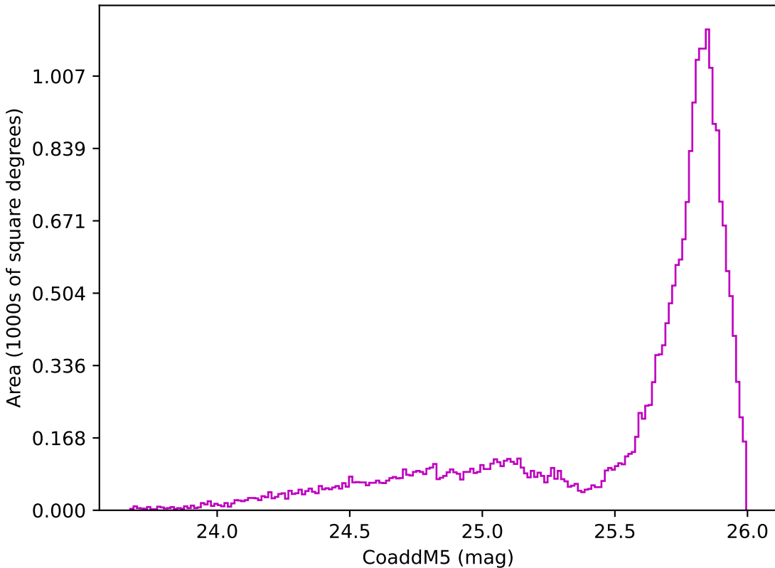
too_ignore_5_4v3.4_10yrs All sky z band: CoaddM5
