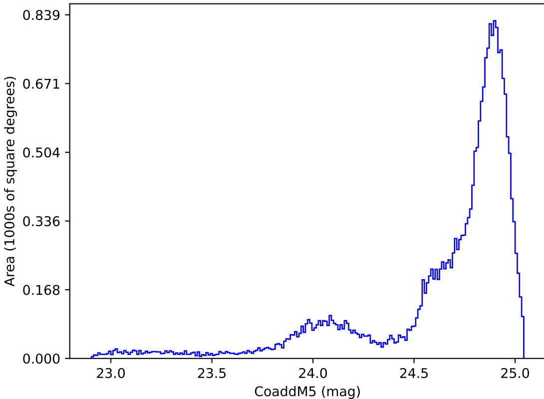
too_ignore_5_4v3.4_10yrs All sky y band: CoaddM5
