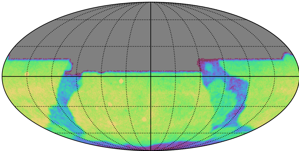
too_ignore_5_4v3.4_10yrs All sky u band: CoaddM5
