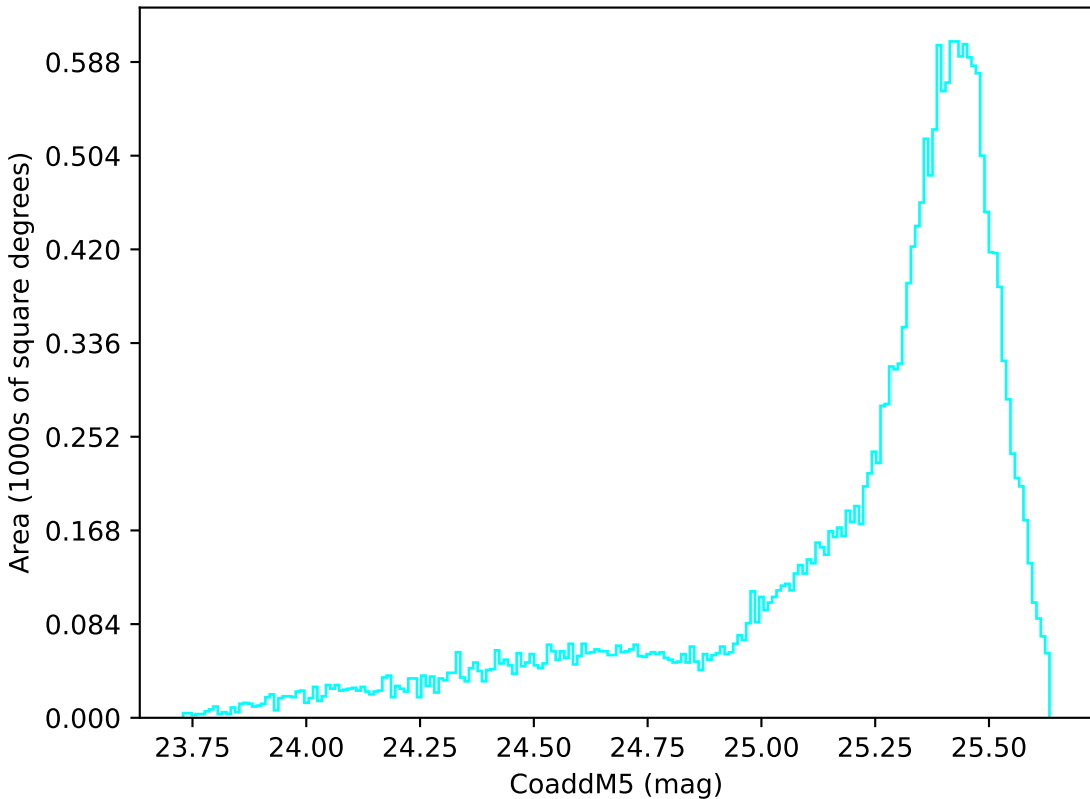
too_ignore_5_4v3.4_10yrs All sky u band: CoaddM5
