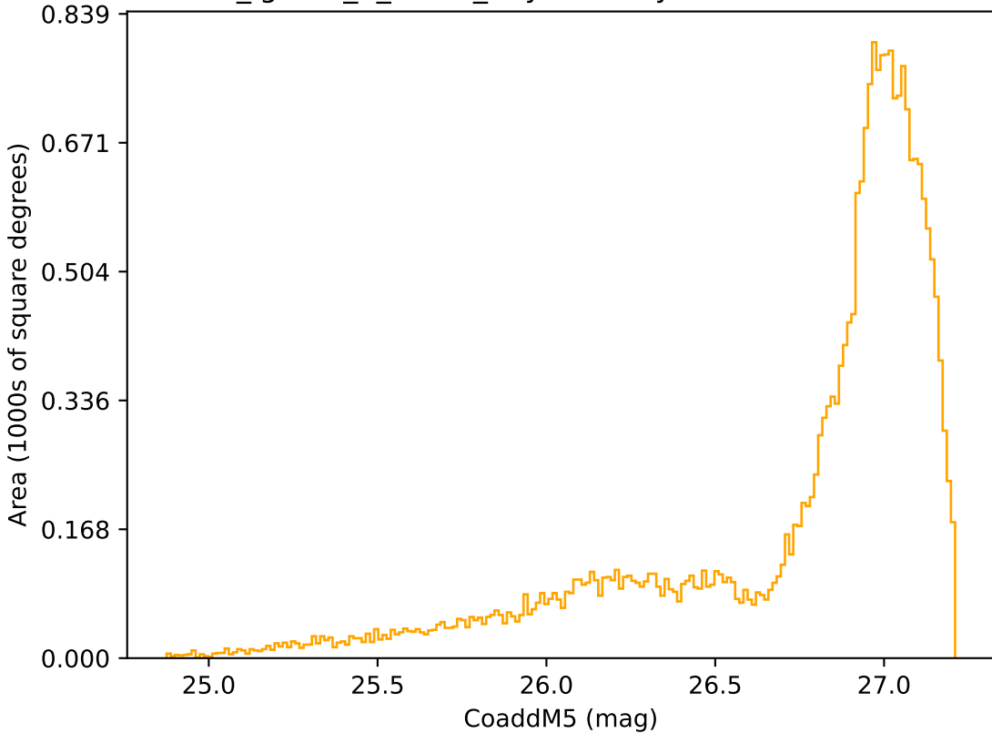
too_ignore_5_4v3.4_10yrs All sky r band: CoaddM5
