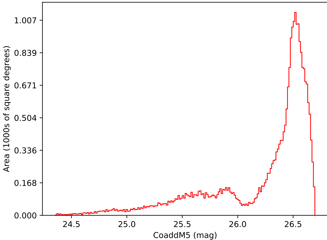
too_ignore_5_4v3.4_10yrs All sky i band: CoaddM5
