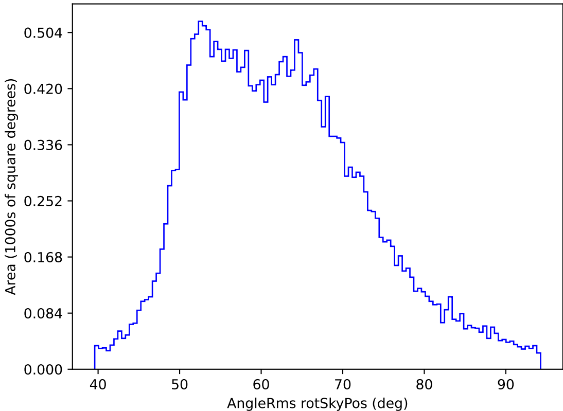
too_ignore_5_4v3.4_10yrs All sky z band: AngleRms rotSkyPos
