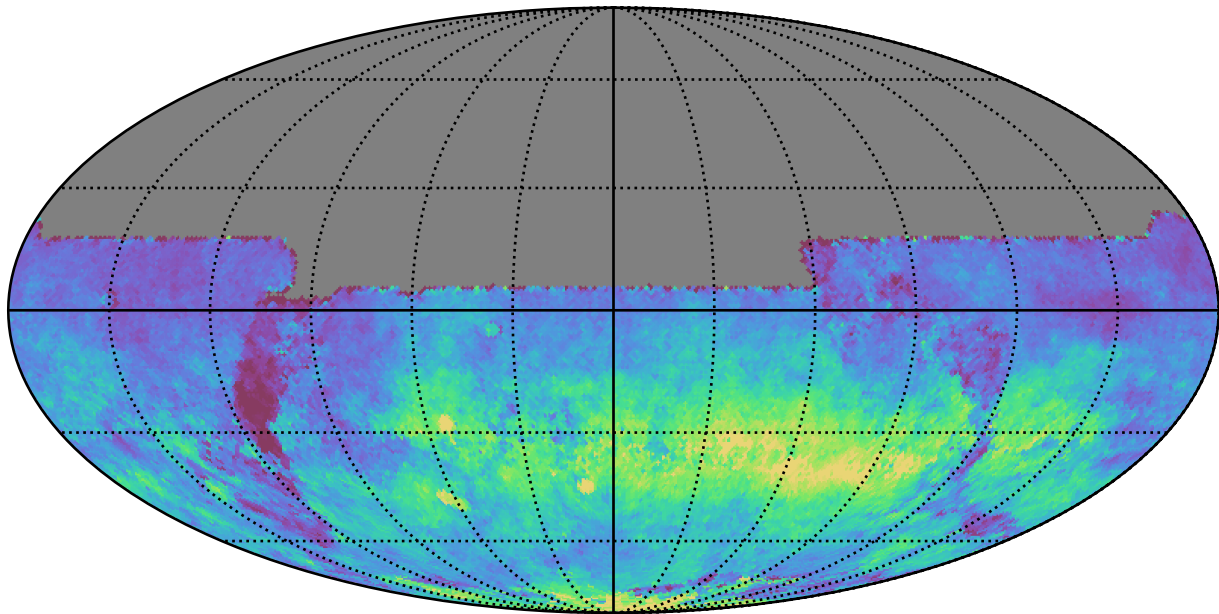
too_ignore_5_4v3.4_10yrs All sky y band: AngleRms rotSkyPos
