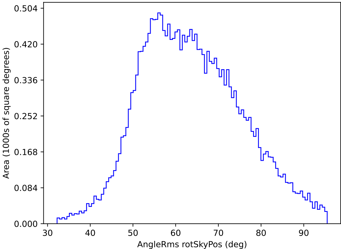
too_ignore_5_4v3.4_10yrs All sky u band: AngleRms rotSkyPos
