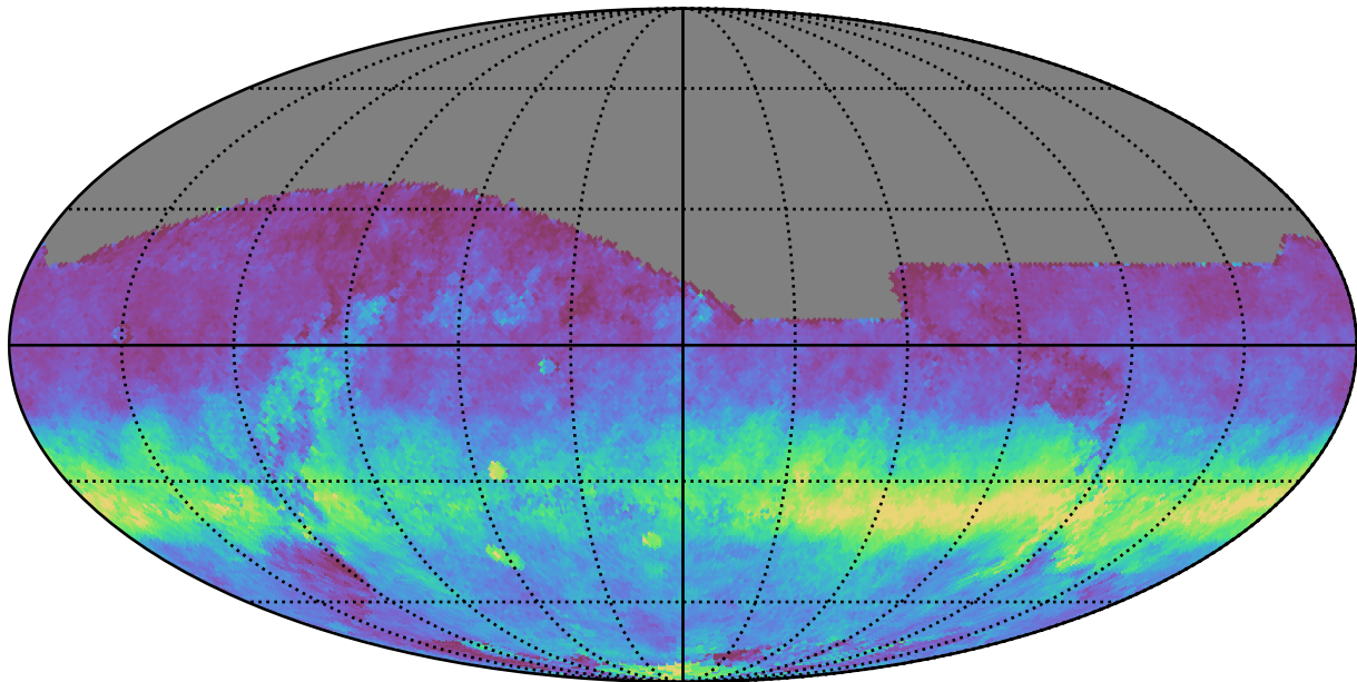
too_ignore_5_4v3.4_10yrs All sky r band: AngleRms rotSkyPos
