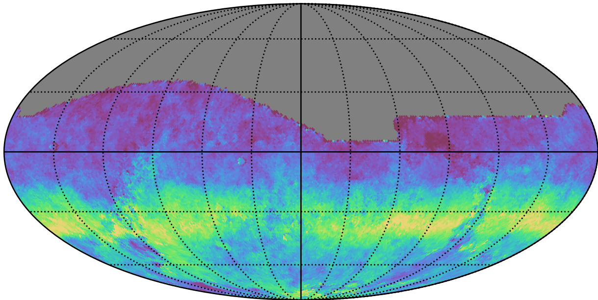
too_ignore_5_4v3.4_10yrs All sky g band: AngleRms rotSkyPos
