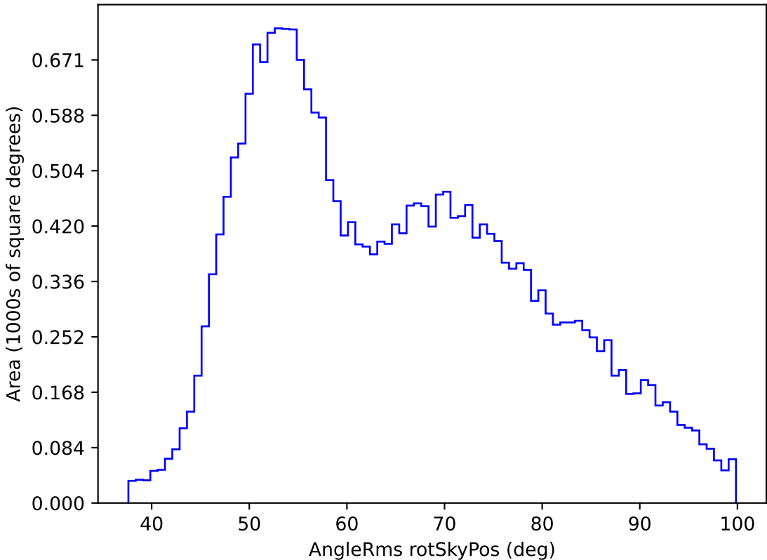
too_ignore_5_4v3.4_10yrs All sky g band: AngleRms rotSkyPos
