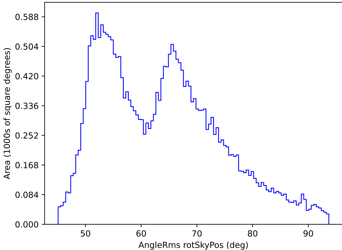
too_ignore_5_4v3.4_10yrs All sky all bands: AngleRms rotSkyPos
