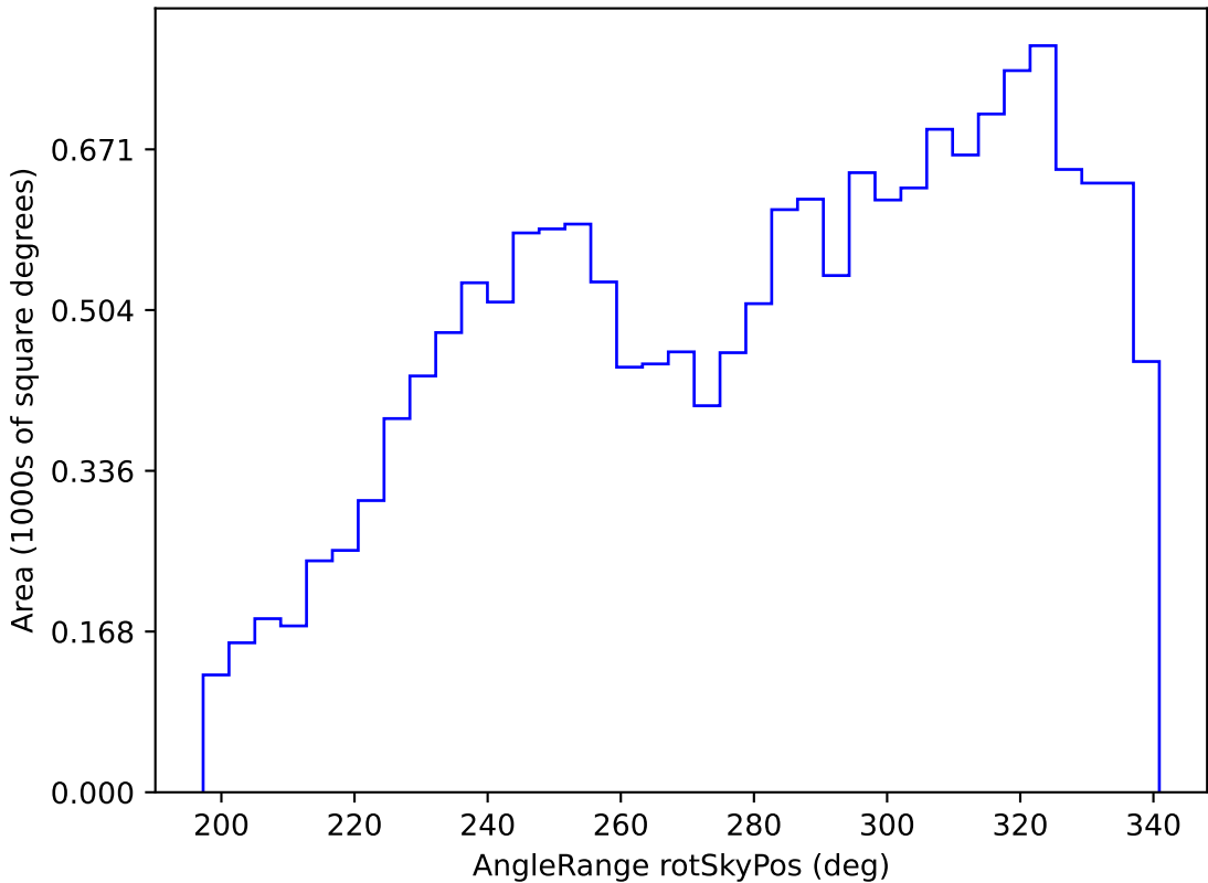
too_ignore_5_4v3.4_10yrs WFD z band: AngleRange rotSkyPos
