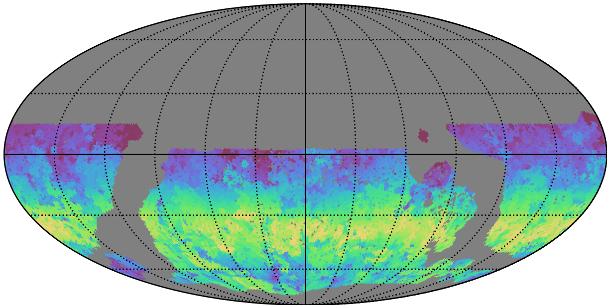
too_ignore_5_4v3.4_10yrs WFD u band: AngleRange rotSkyPos
