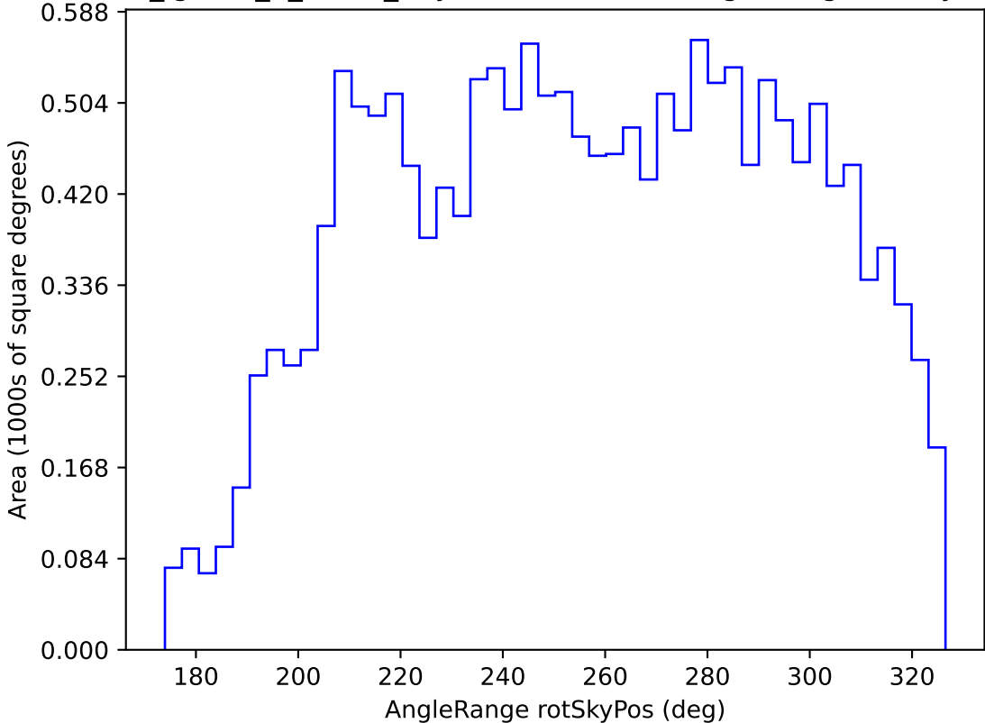
too_ignore_5_4v3.4_10yrs WFD u band: AngleRange rotSkyPos
