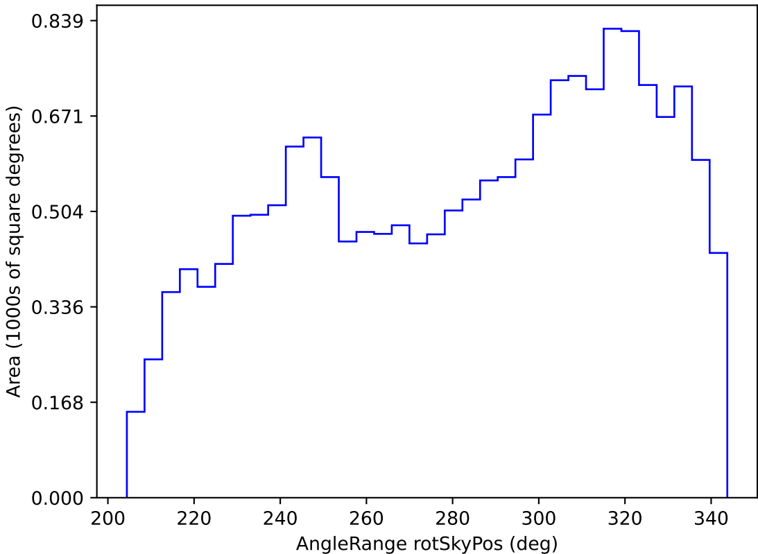
too_ignore_5_4v3.4_10yrs WFD r band: AngleRange rotSkyPos
