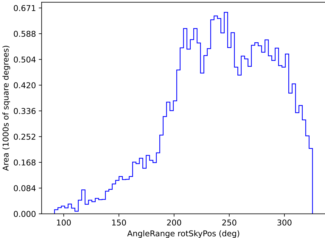
too_ignore_5_4v3.4_10yrs All sky u band: AngleRange rotSkyPos
