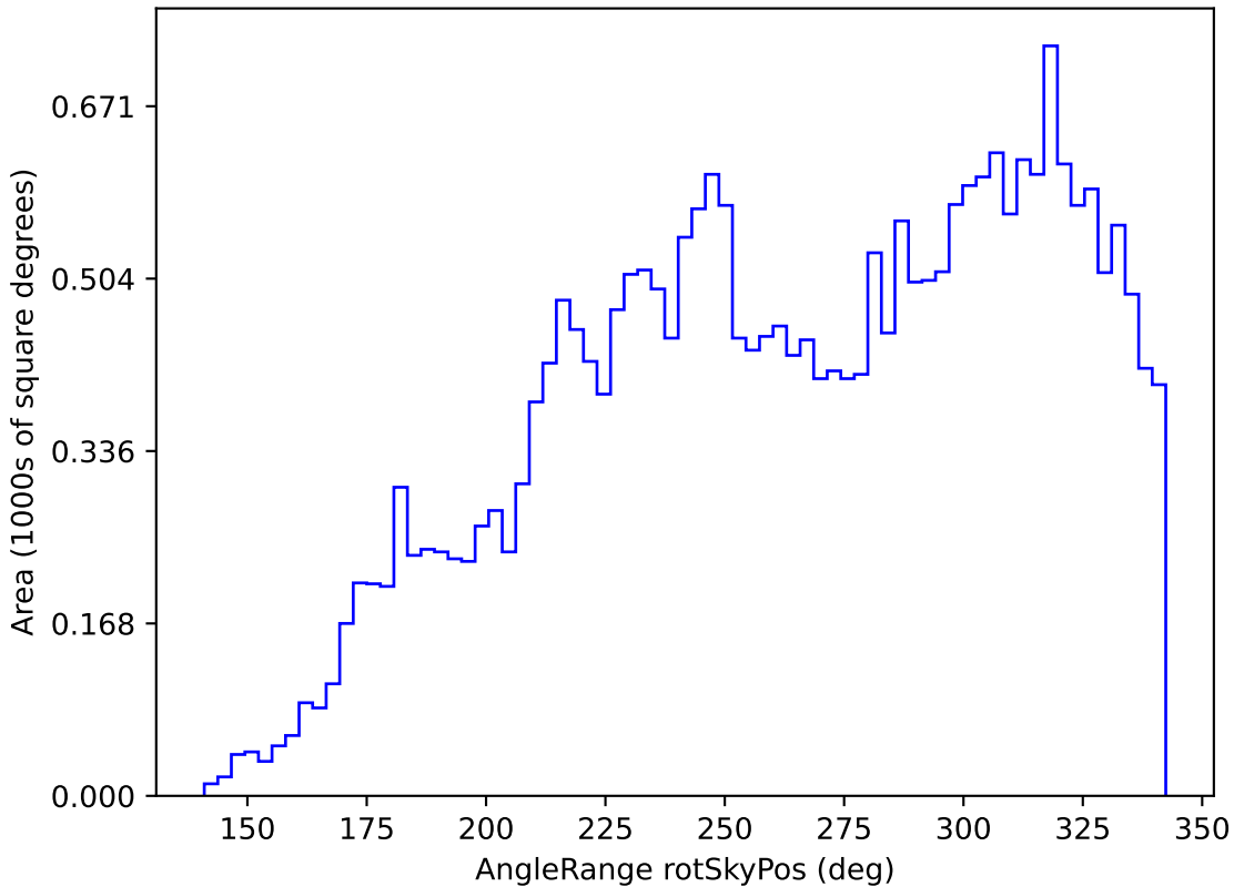
too_ignore_5_4v3.4_10yrs All sky r band: AngleRange rotSkyPos
