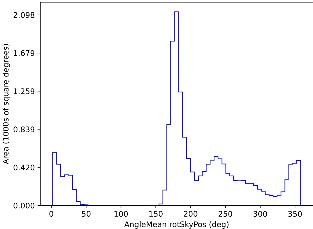
too_ignore_5_4v3.4_10yrs WFD r band: AngleMean rotSkyPos
