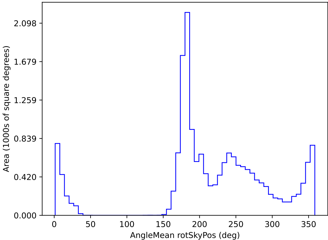
too_ignore_5_4v3.4_10yrs WFD i band: AngleMean rotSkyPos
