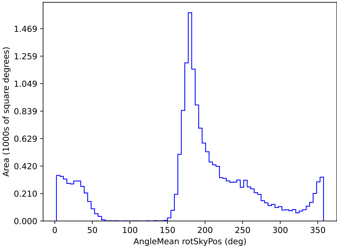
too_ignore_5_4v3.4_10yrs WFD g band: AngleMean rotSkyPos
