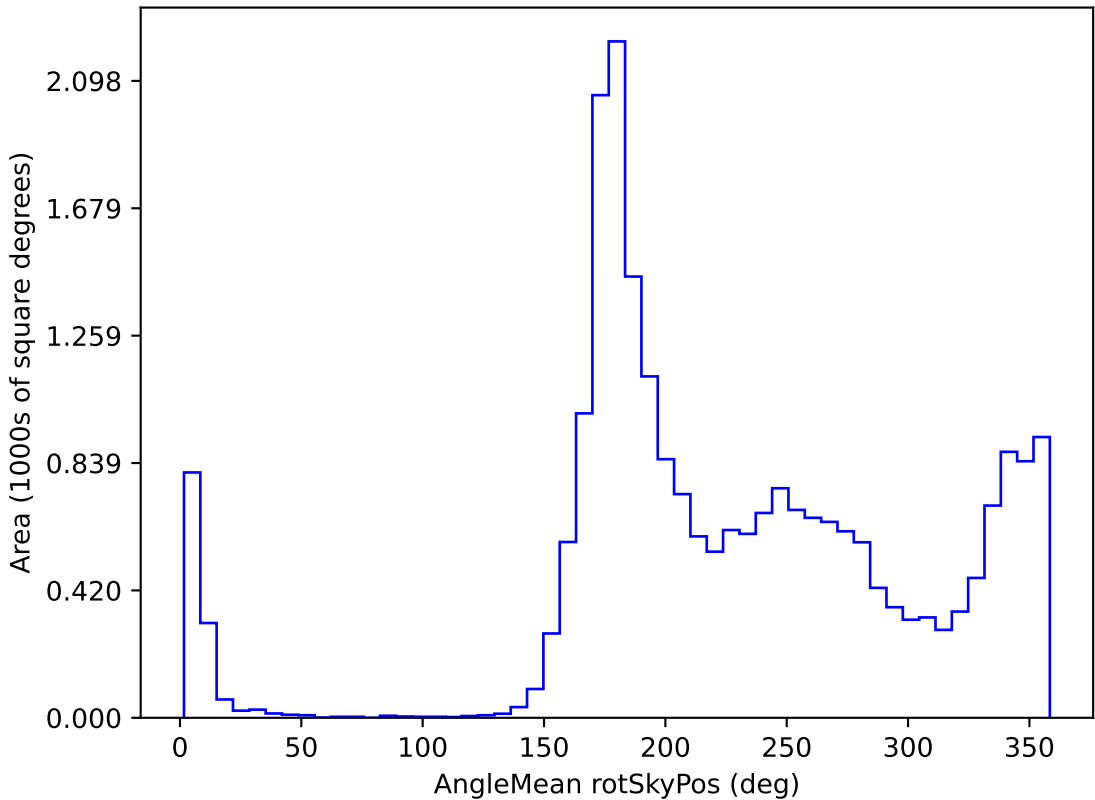
too_ignore_5_4v3.4_10yrs All sky y band: AngleMean rotSkyPos
