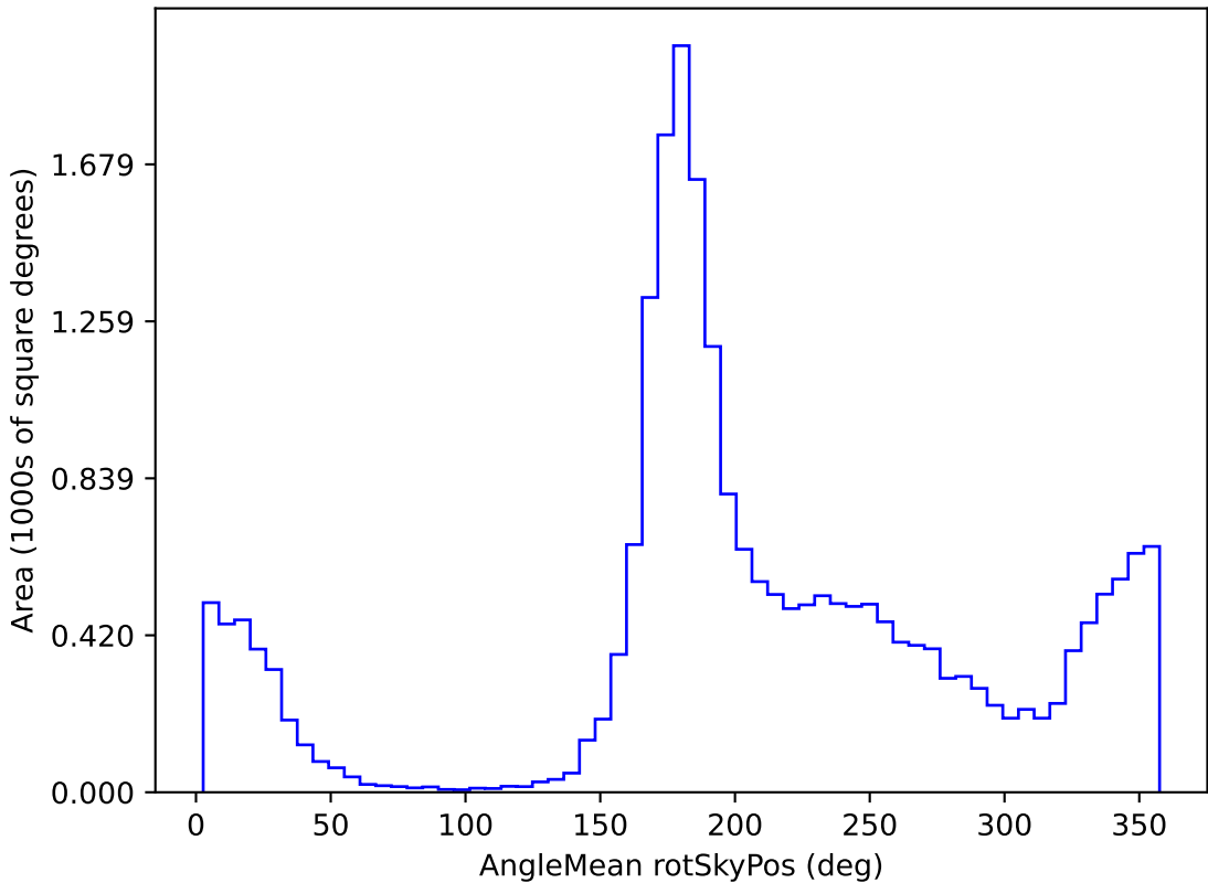
too_ignore_5_4v3.4_10yrs All sky u band: AngleMean rotSkyPos
