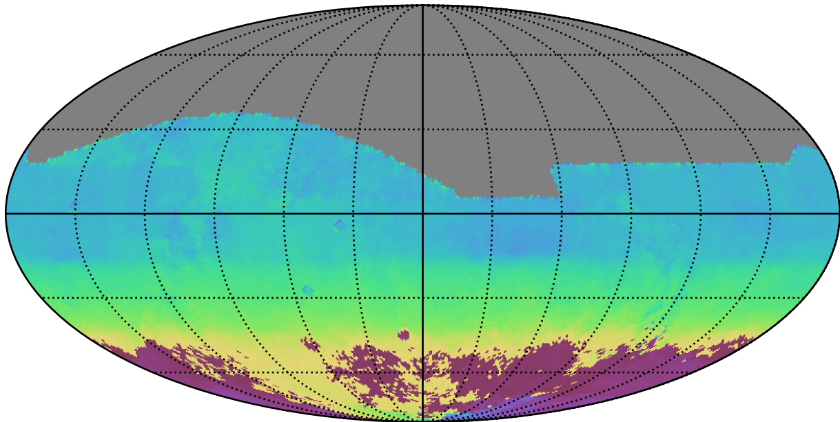
too_ignore_5_4v3.4_10yrs All sky i band: AngleMean rotSkyPos
