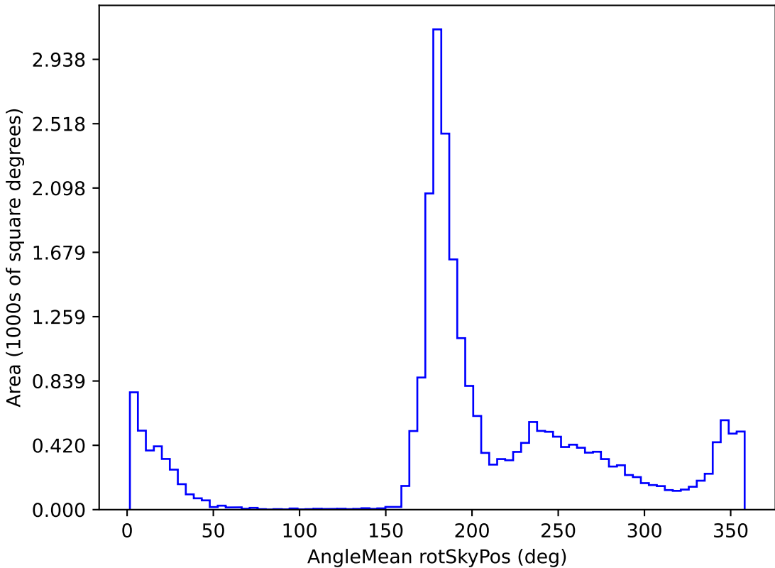
too_ignore_5_4v3.4_10yrs All sky all bands: AngleMean rotSkyPos
