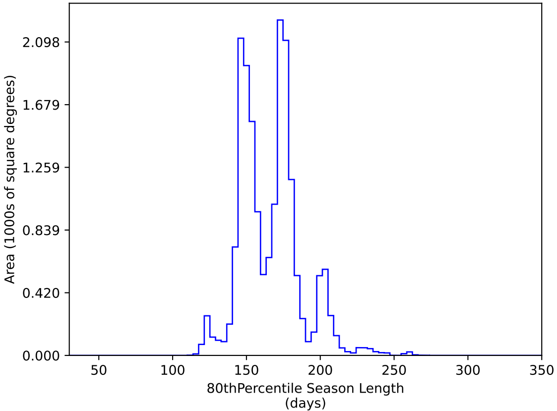
too_ignore_5_4v3.4_10yrs WFD y band: 80thPercentile Season Length
