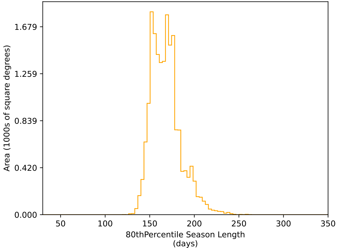
too_ignore_5_4v3.4_10yrs WFD r band: 80thPercentile Season Length
