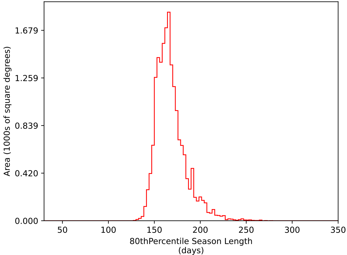
too_ignore_5_4v3.4_10yrs WFD i band: 80thPercentile Season Length
