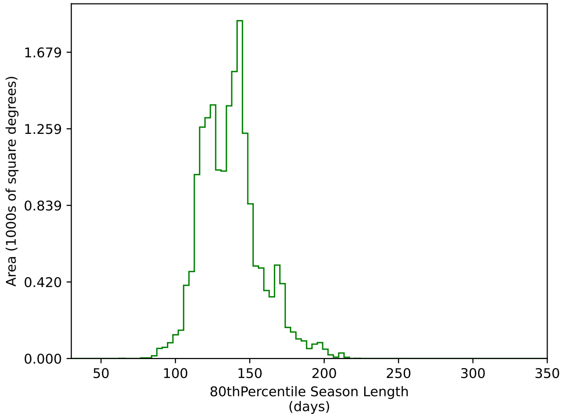
too_ignore_5_4v3.4_10yrs WFD g band: 80thPercentile Season Length
