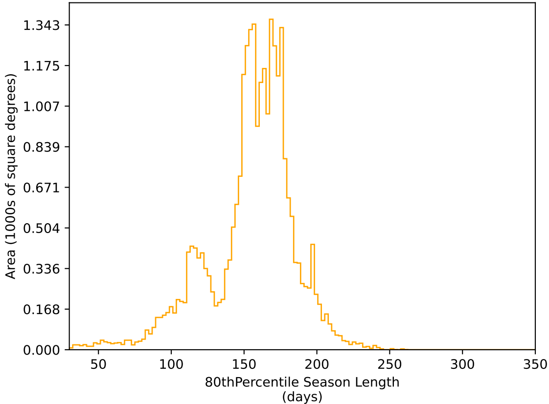
too_ignore_5_4v3.4_10yrs All sky r band: 80thPercentile Season Length
