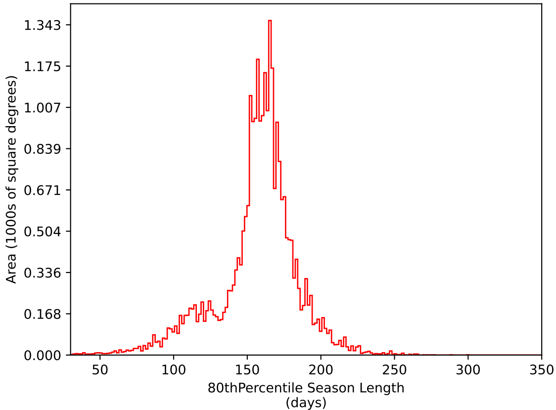
too_ignore_5_4v3.4_10yrs All sky i band: 80thPercentile Season Length
