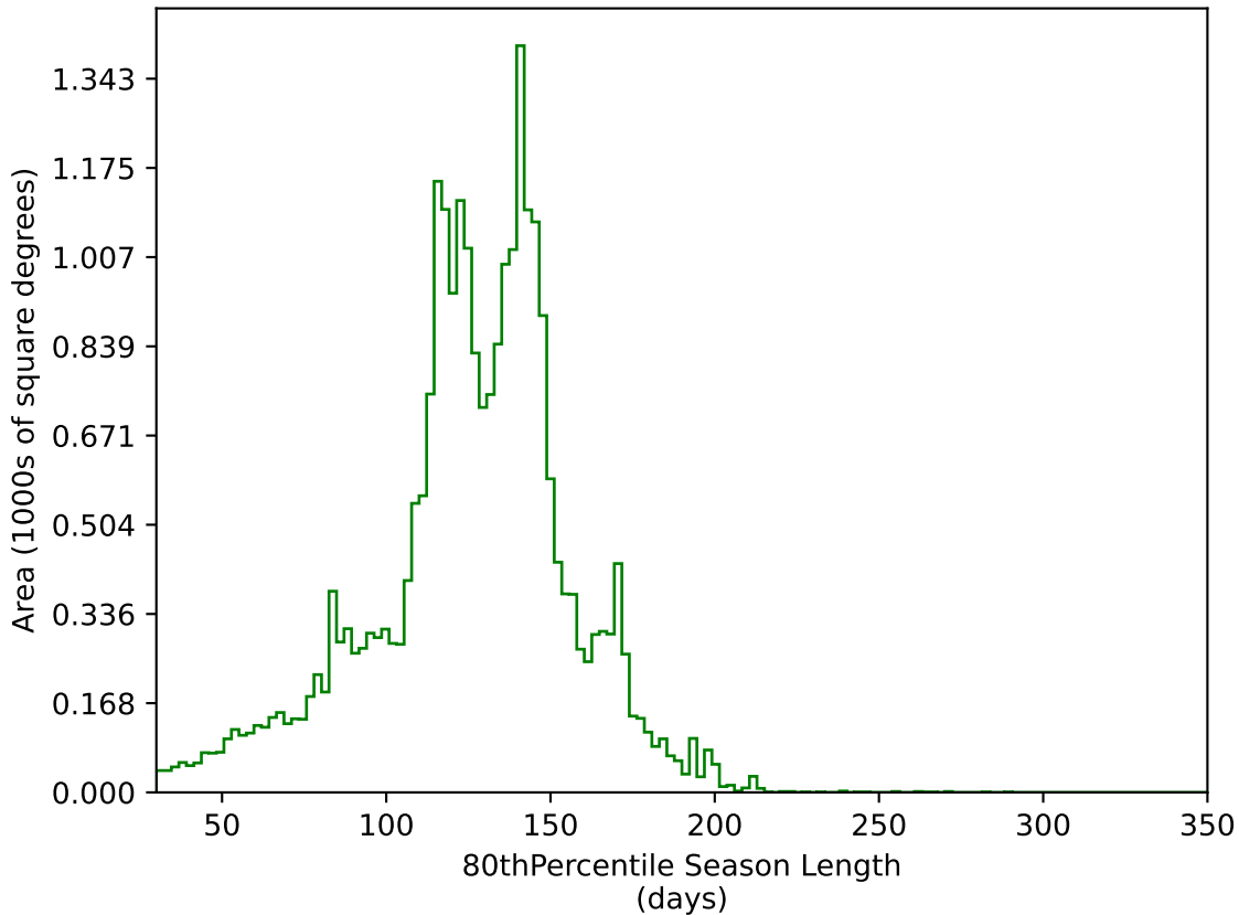
too_ignore_5_4v3.4_10yrs All sky g band: 80thPercentile Season Length
