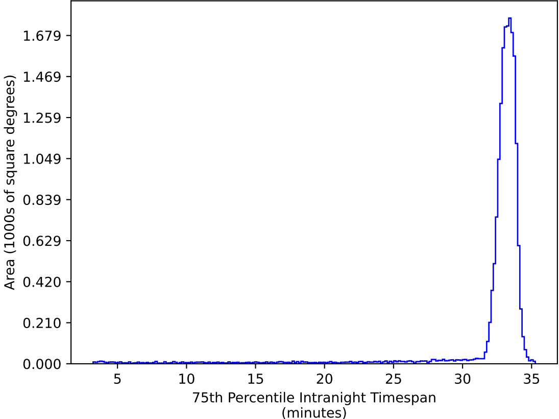
too_ignore_5_4v3.4_10yrs WFD ug bands: 75th Percentile Intranight Timespan
