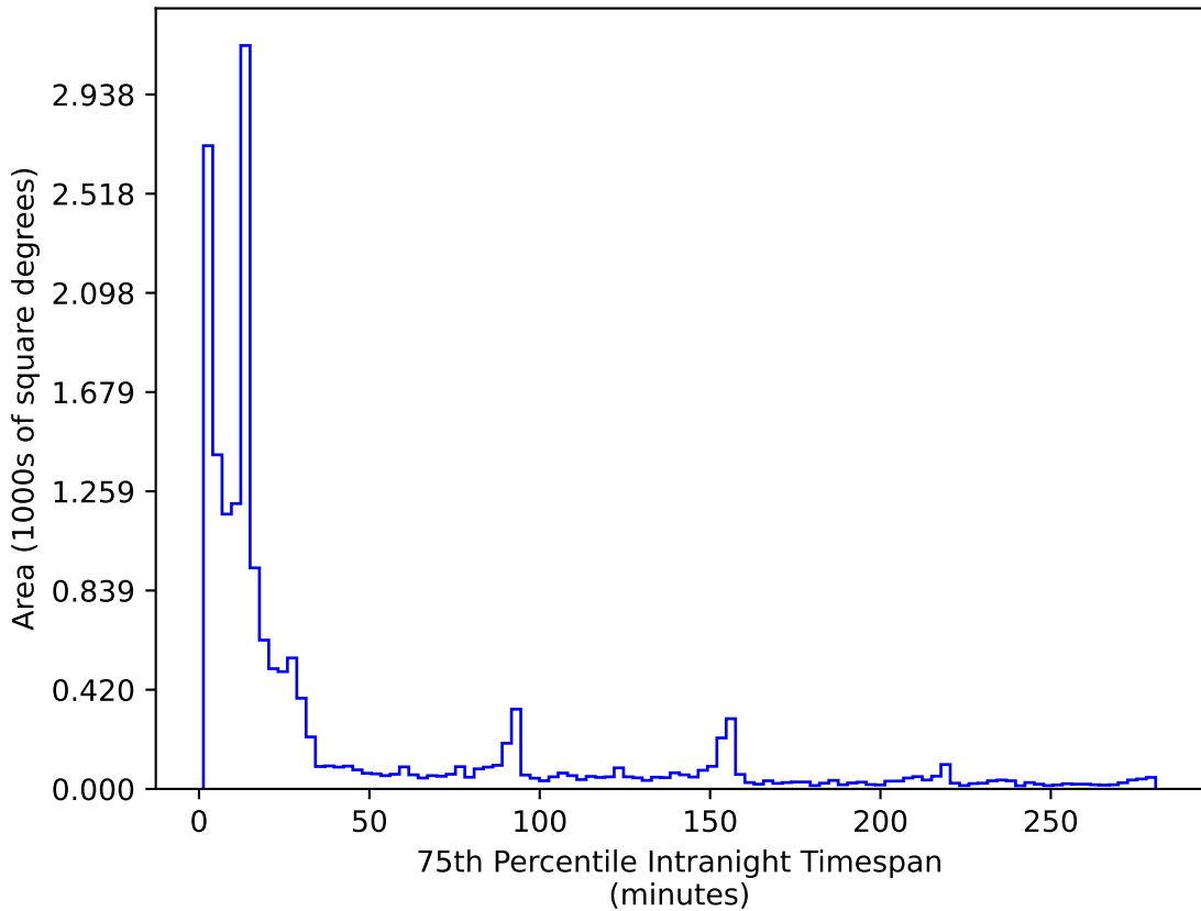
too_ignore_5_4v3.4_10yrs WFD r band: 75th Percentile Intranight Timespan
