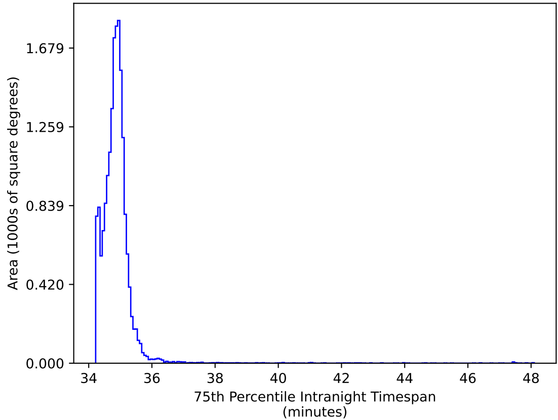
too_ignore_5_4v3.4_10yrs WFD iz bands: 75th Percentile Intranight Timespan
