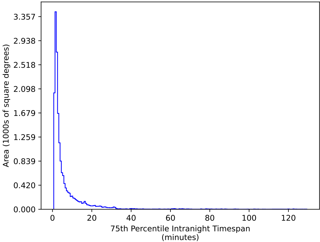
too_ignore_5_4v3.4_10yrs WFD g band: 75th Percentile Intranight Timespan
