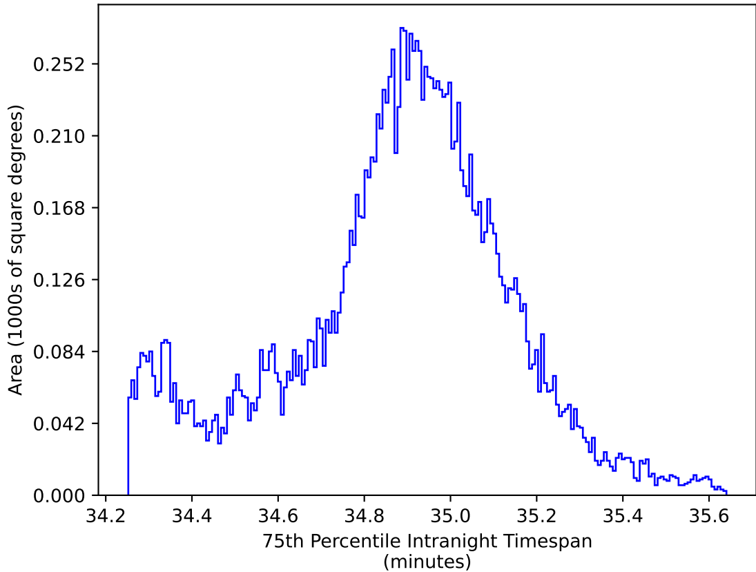
too_ignore_5_4v3.4_10yrs WFD all bands: 75th Percentile Intranight Timespan
