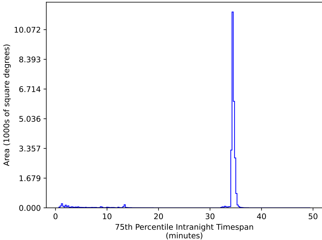
too_ignore_5_4v3.4_10yrs All sky zy bands: 75th Percentile Intranight Timespan
