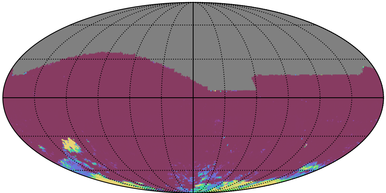
too_ignore_5_4v3.4_10yrs All sky ri bands: 75th Percentile Intranight Timespan
