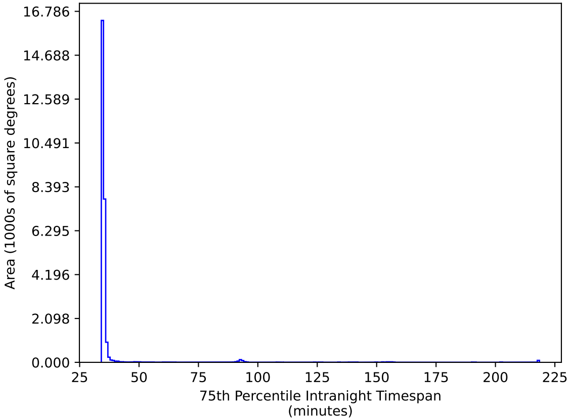
too_ignore_5_4v3.4_10yrs All sky ri bands: 75th Percentile Intranight Timespan
