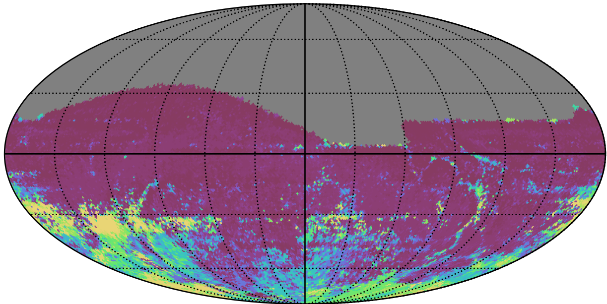
too_ignore_5_4v3.4_10yrs All sky r band: 75th Percentile Intranight Timespan
