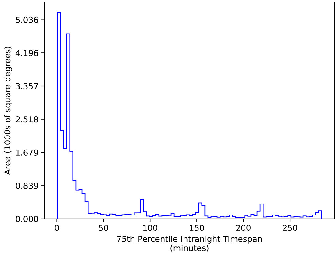
too_ignore_5_4v3.4_10yrs All sky r band: 75th Percentile Intranight Timespan
