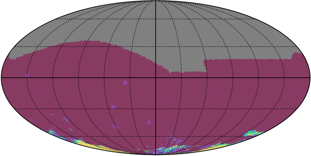
too_ignore_5_4v3.4_10yrs All sky iz bands: 75th Percentile Intranight Timespan
