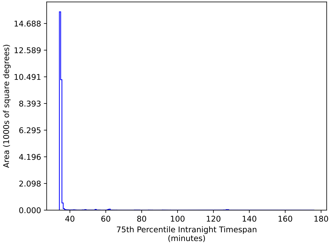
too_ignore_5_4v3.4_10yrs All sky iz bands: 75th Percentile Intranight Timespan
