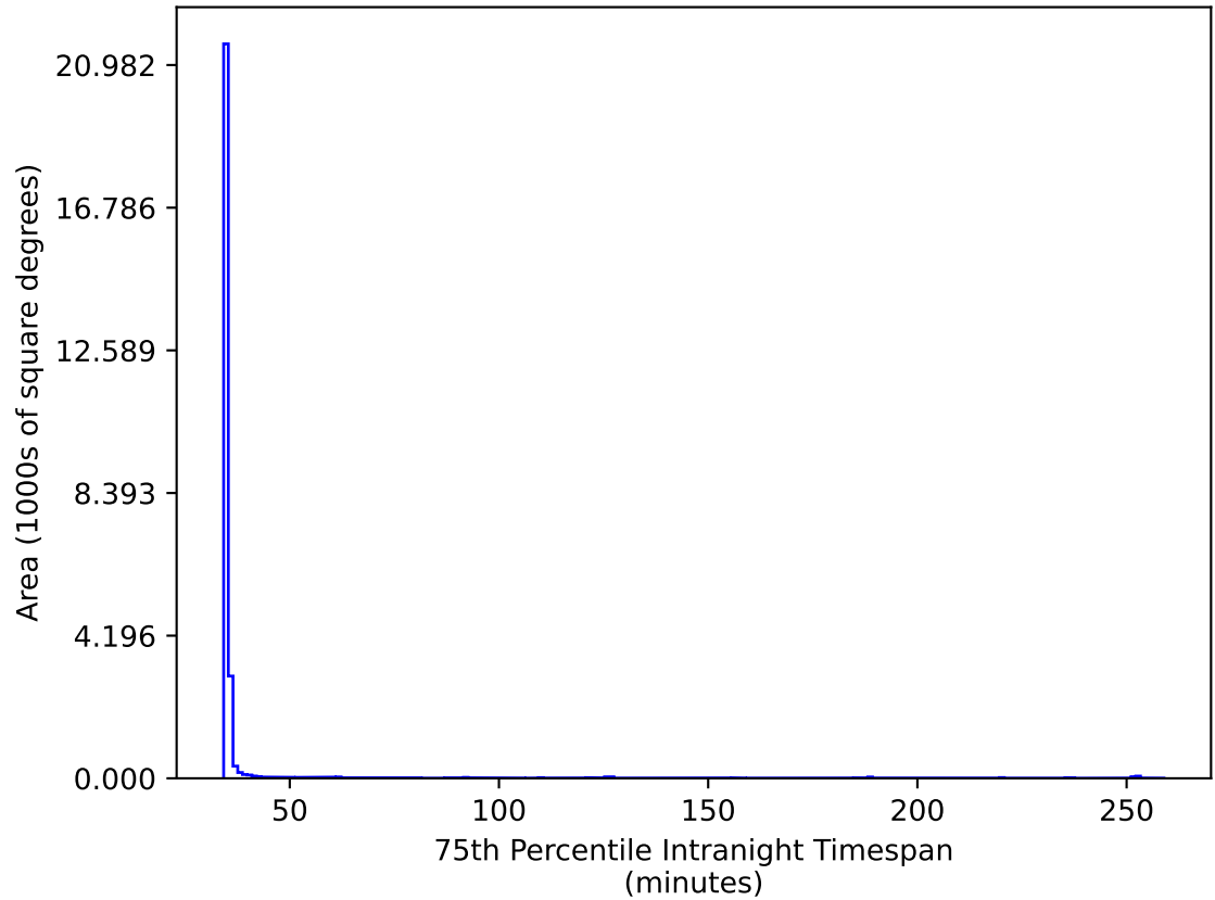
too_ignore_5_4v3.4_10yrs All sky gr bands: 75th Percentile Intranight Timespan
