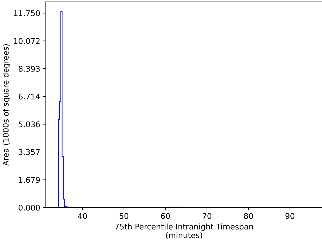
too_ignore_5_4v3.4_10yrs All sky all bands: 75th Percentile Intranight Timespan
