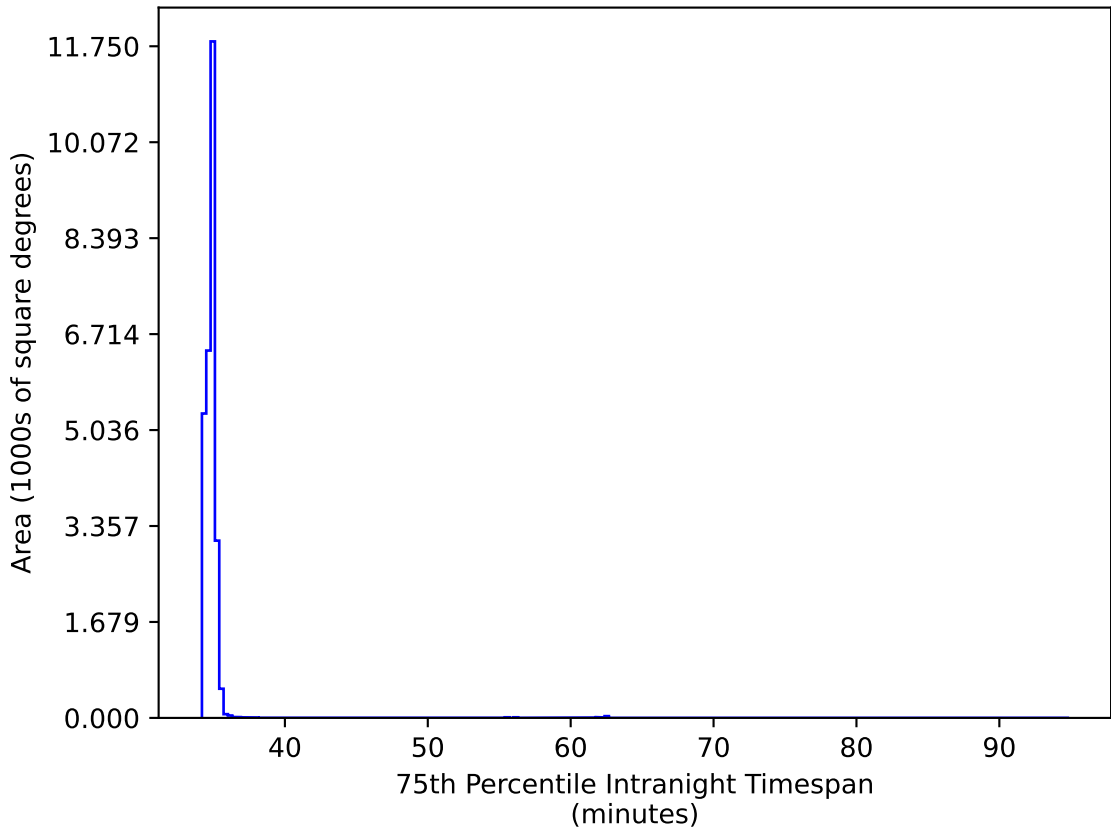
too_ignore_5_4v3.4_10yrs All sky: 75th Percentile Intranight Timespan
